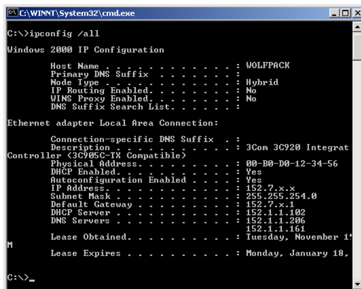
Figure 8: one of the output of ipConfig command.
