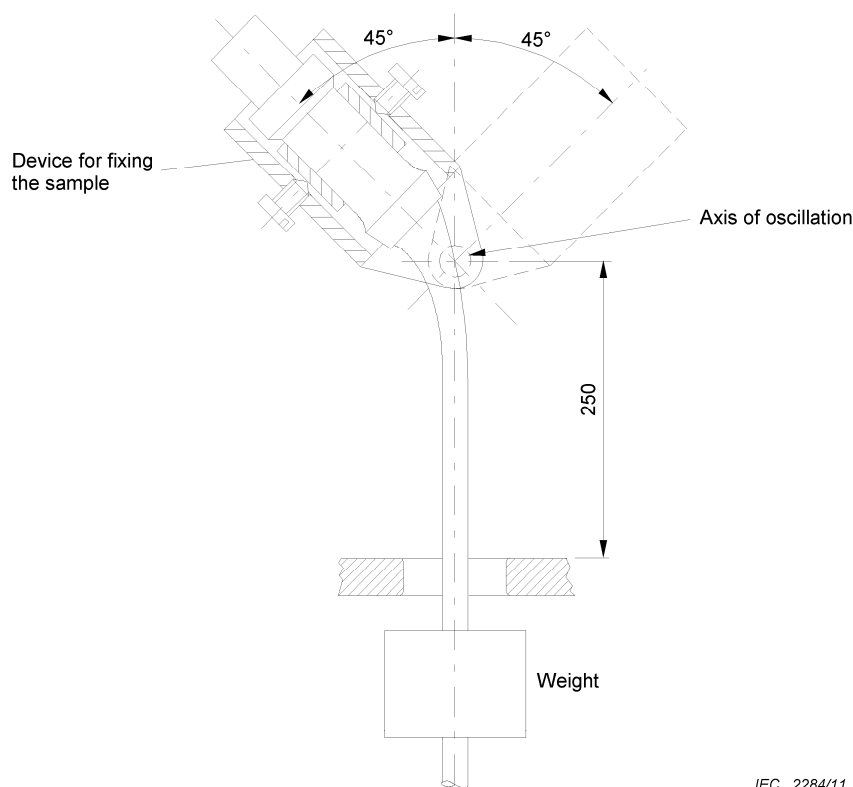
Figure 14 – Apparatus for flexing test
