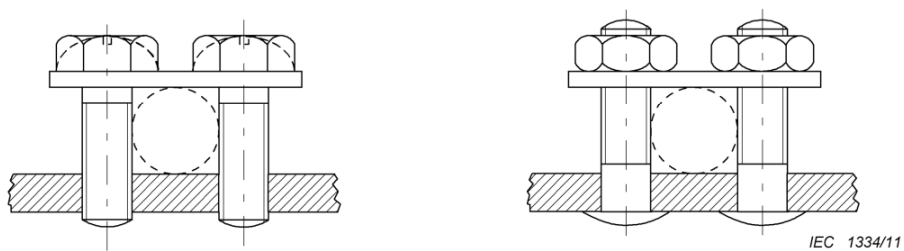
d) Saddle terminals
