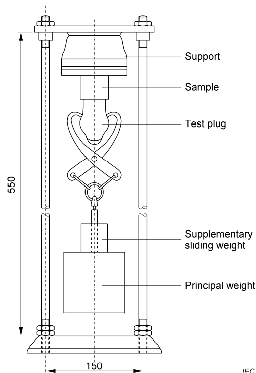
Figure 8 – Apparatus for checking the withdrawal force
