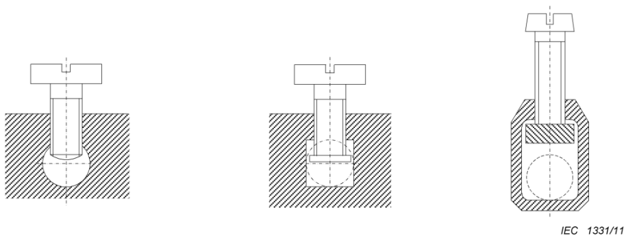
a) Pillar terminals
