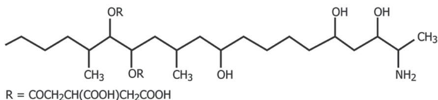
Fumonisin B 1
