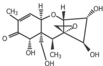
Nivalenol
